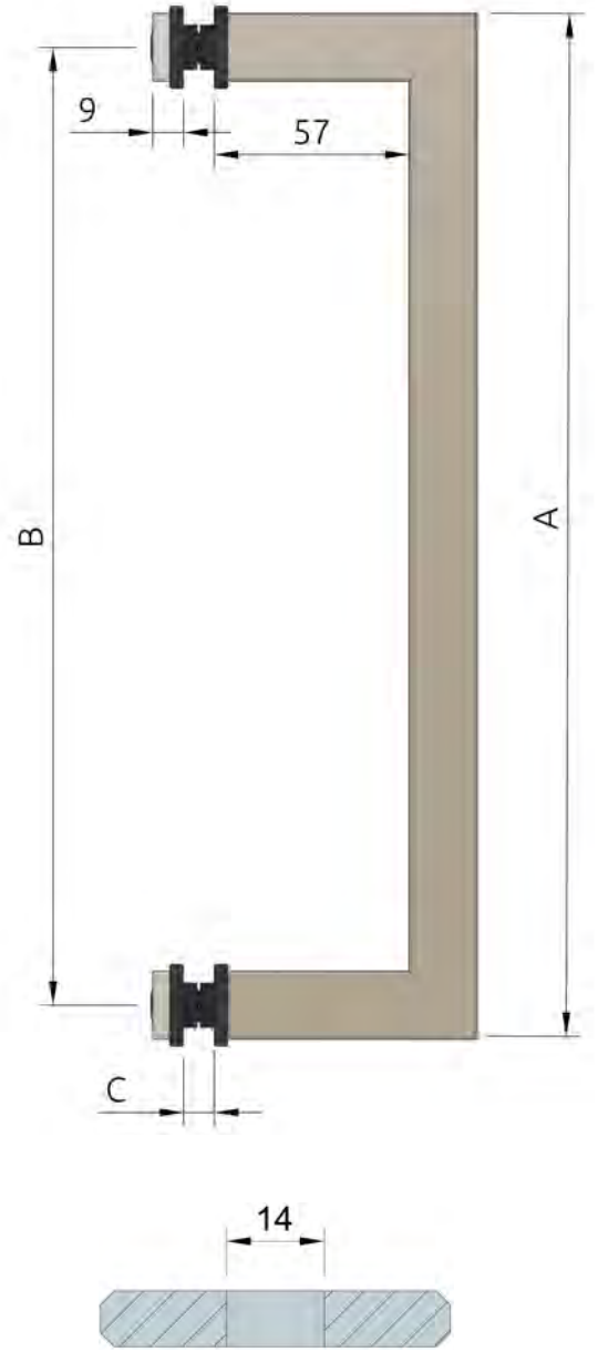
35*20 Cam Kapı Kolu 35*20 Glass Door Handle
