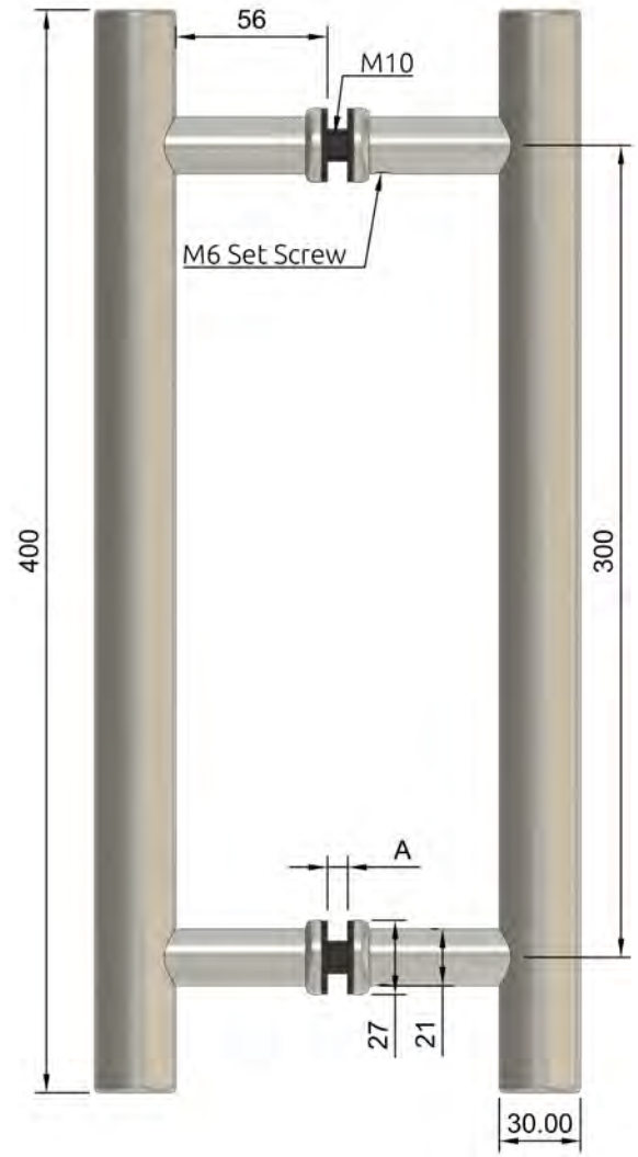
Ø30 400 mm Cam & Alüminyum Kapı Kolu Ø30 400 mm Glass & Aluminium Door Handle
